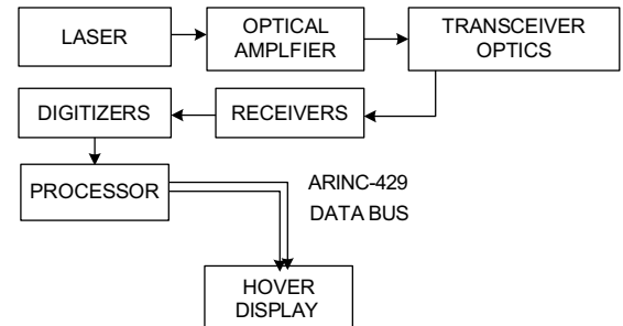
Figure 2 Block diagram
