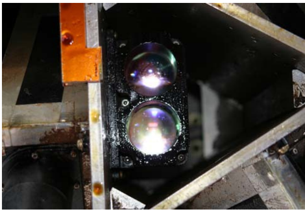
Figure 7 The laser altimeter sensor mounted on the OADS UH-1H. The lenses, coated with a layer of oil and dirt, remained functional throughout the flight test.
