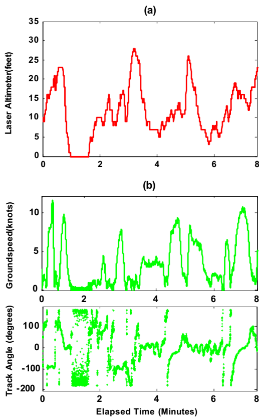
Figure 13 Data from clear air test flight over tarmac; (a) accurate height above ground measurements, and (b)
